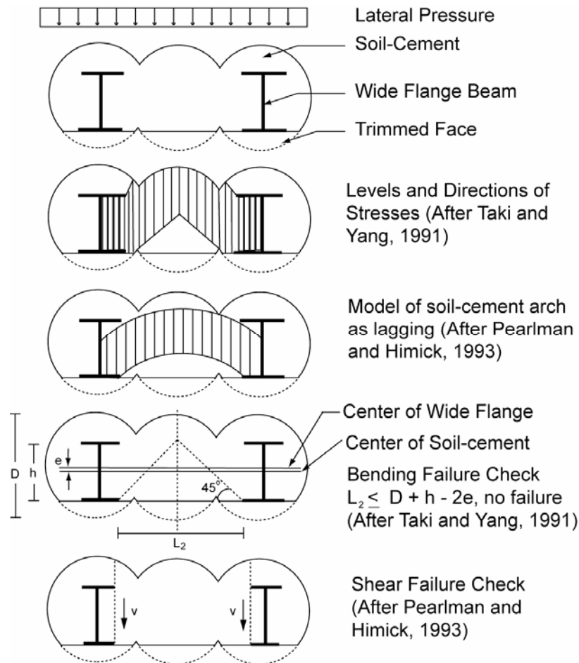
Figure 8. Structural Resistance of Wall Elements.
