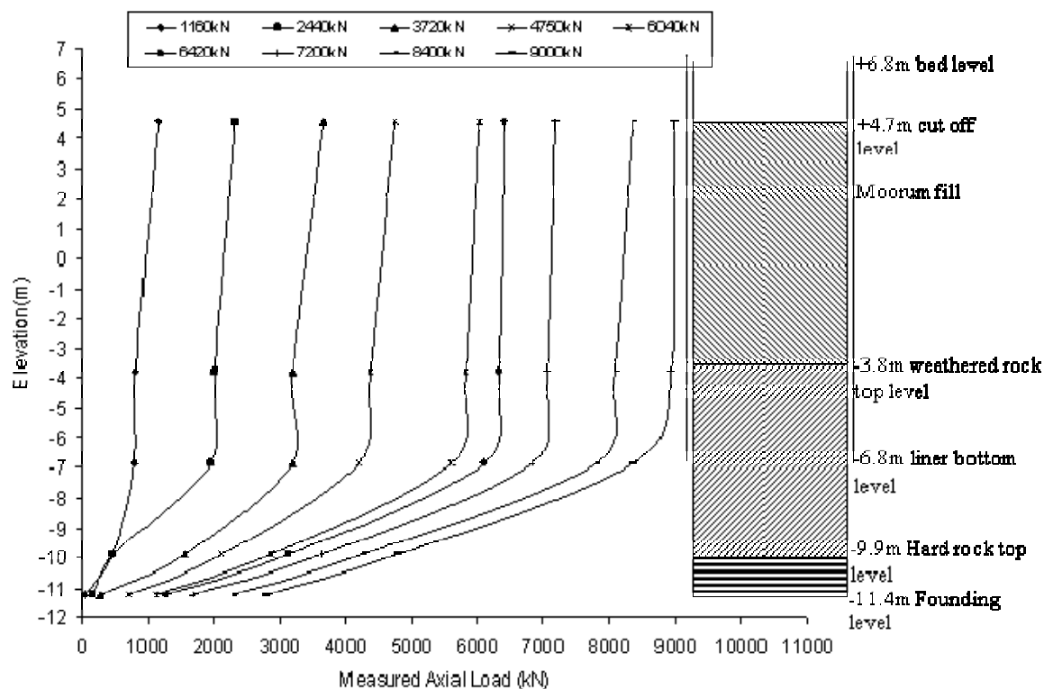
Figure 16. Mobilization of Axial Load.
