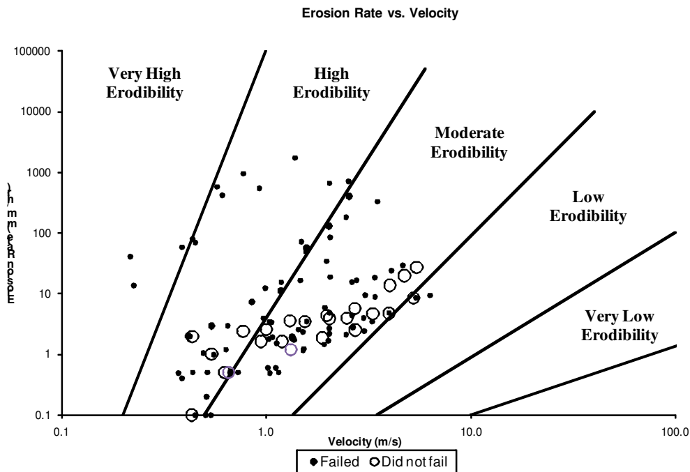
Figure 34. Overtopping comparison of pass vs. fail.
