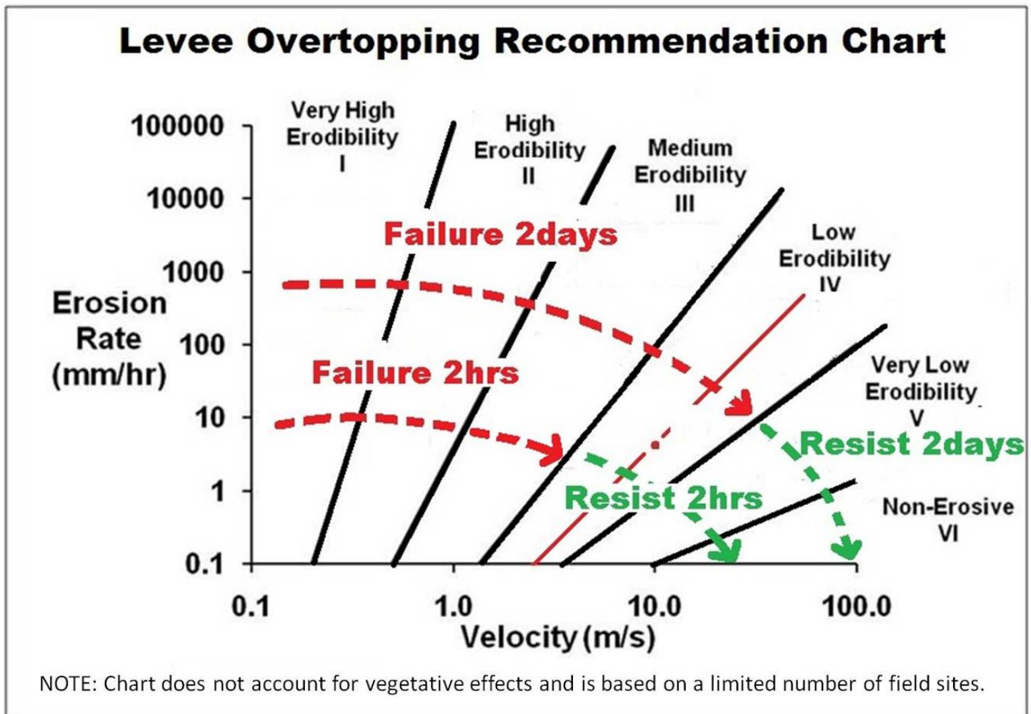
Figure 36. Recommendation chart for overtopping events.
