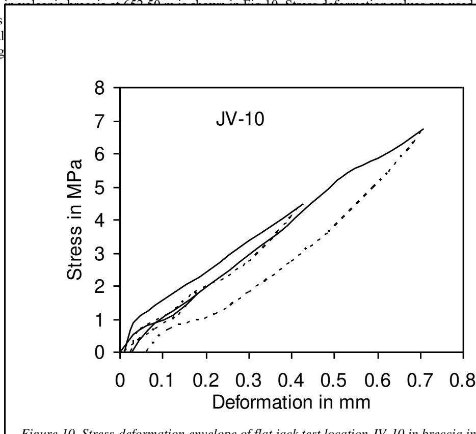
Figure 10. Stress deformation envelope of flat jack test location JV-10 in breccia in pilot shaft.
