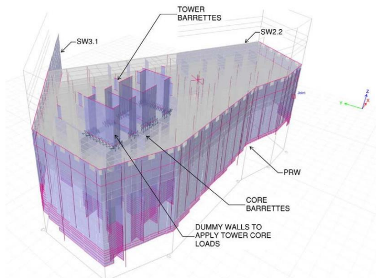
Figure 10. Snapshot of structural model.
