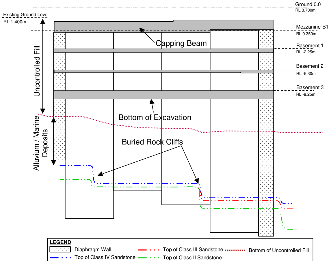
Figure 7. A typical section of the ground profile at Site location – Section C-C.
