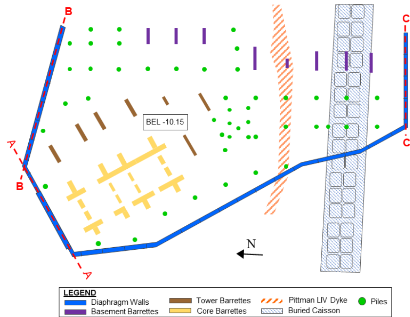
Figure 2. Crown Sydney Hotel Resort basement foundation plan.
