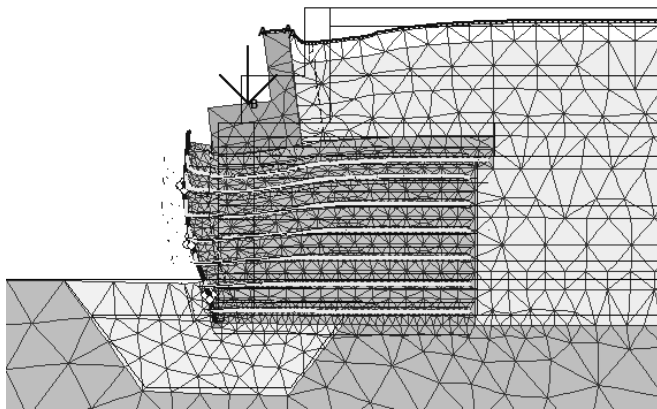
Figure 14. Deformed mesh (a) and shear strains (b) at post-construction serviceability stages. Base case.
