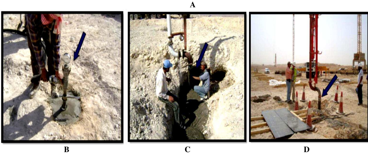
Figure 9.a. and b. Karst foundation bedrock treatments; cement grout injection, c. and d. high slump concrete filling.
