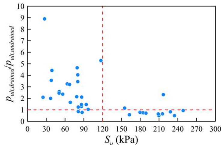
Fig. 6 – Plot of p_{ult,drained}/p_{ult,undrained} vs S_u for Houston, Texas, soil data (36 data points).
