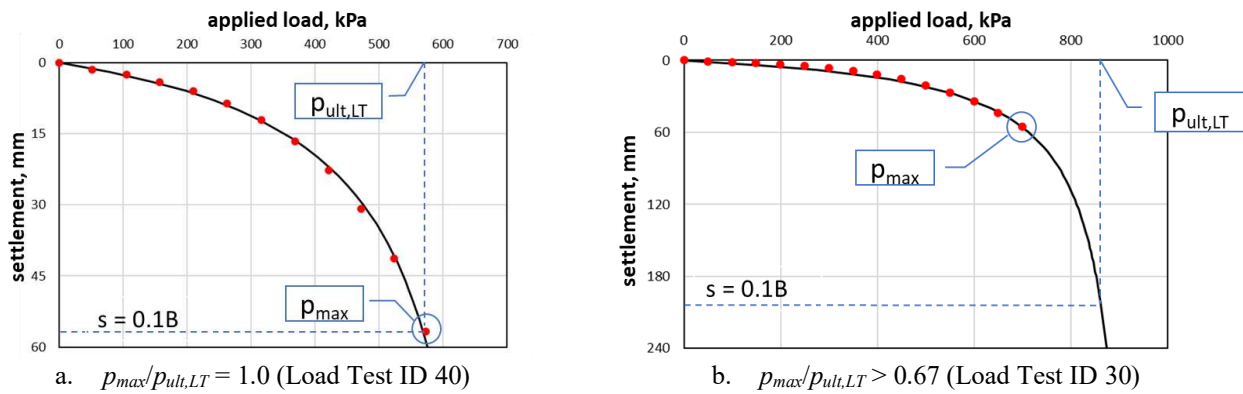
Fig. 1 – p_{ult} , measured from load settlement curve: a) read directly from the load settlement curve; b) extrapolated from the load settlement curve.
