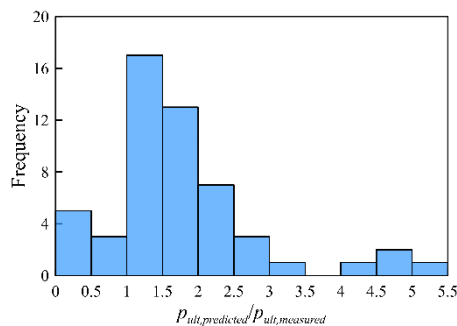
c. Histogram for AASHTO/FHWA bearing capacity factors.
