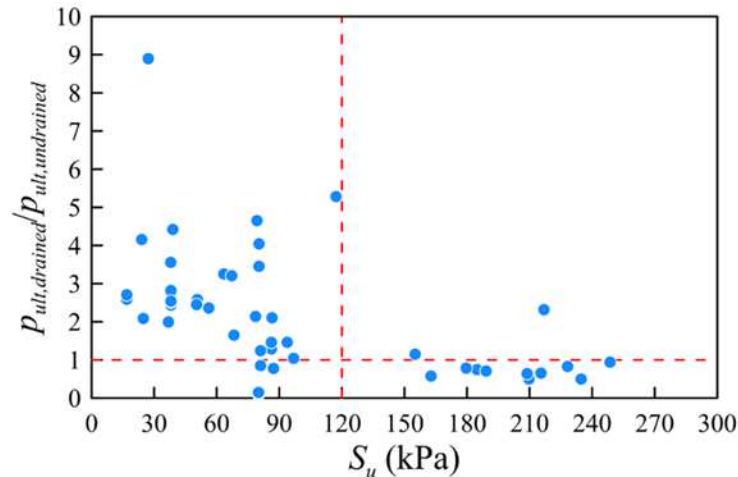
Fig. 7 – Plot of p_{ult,drained}/p_{ult,undrained} vs. S_u for combined TAMU-SHAL-CLAY-Load Test information and Houston, Texas, soil data (64 data points).
