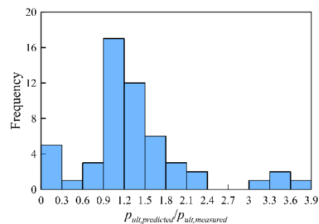
d. Histogram for Briaud (2023) bearing capacity factors.
