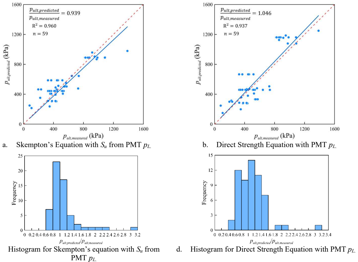
Fig. 4 - Comparison of p_{ult,measured} and p_{ult,predicted} : a) using Skempton's equation with S_u correlated with PMT p_L ; b) using direct strength equation with PMT p_L ; c) histogram of p_{ult,predicted}/p_{ult,measured} for S_u correlated with PMT p_L ; and d) histogram of p_{ult,predicted}/p_{ult,measured} for direct strength equation with PMT p_L .
