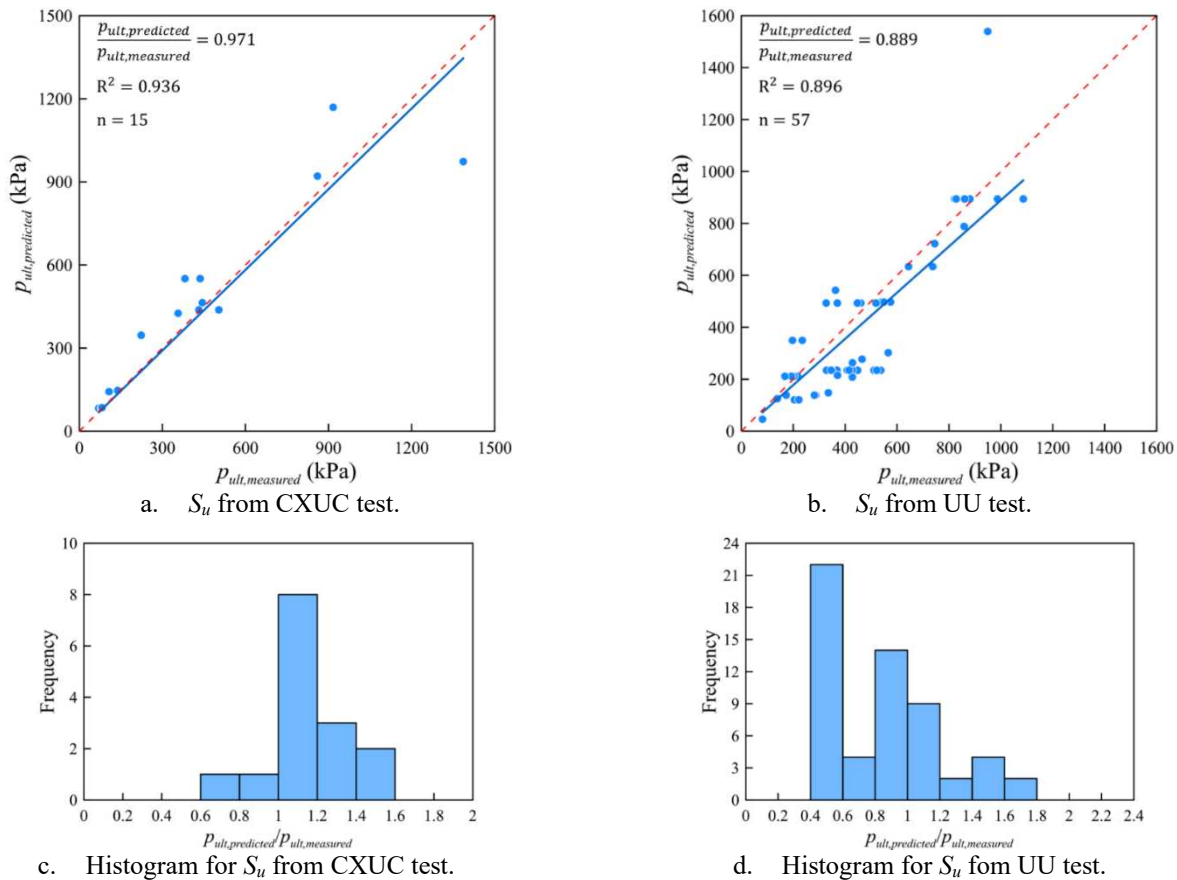
Fig. 3 - Comparison of p_{ult,measured} and p_{ult,predicted} using Skempton's equation: a) with S_u from a CXUC test; b) with S_u from a UU test; c) histogram of p_{ult,predicted}/p_{ult,measured} for S_u from CXUC test; and d) histogram of p_{ult,predicted}/p_{ult,measured} for S_u from UU test.
